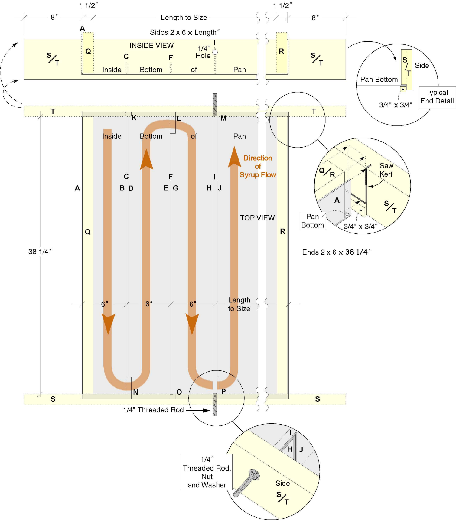
Typical Side Detail Rotated 90°
