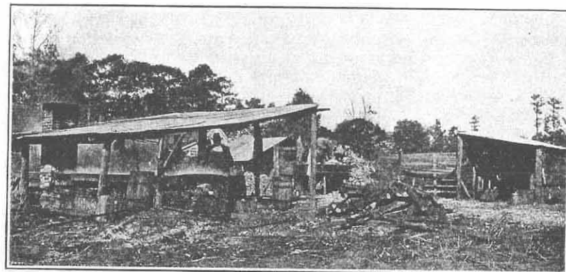
FIG. 13.—A sirup-making outfit for a farm producing 5 to 15 acres of cane. This has a capacity of about 200 gallons of sirup a day. The mill is operated by a 6-horsepower gasoline engine. The evaporator uses wood for fuel. The cost of the outfit at pre-war prices was about $600
