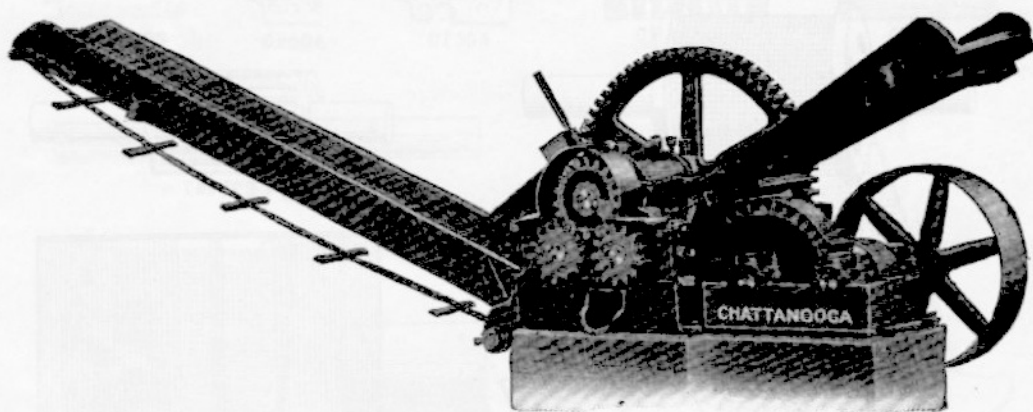
No. 145-A Belt-Power Cane Mill. (The bagasse carrier is extra equipment)
