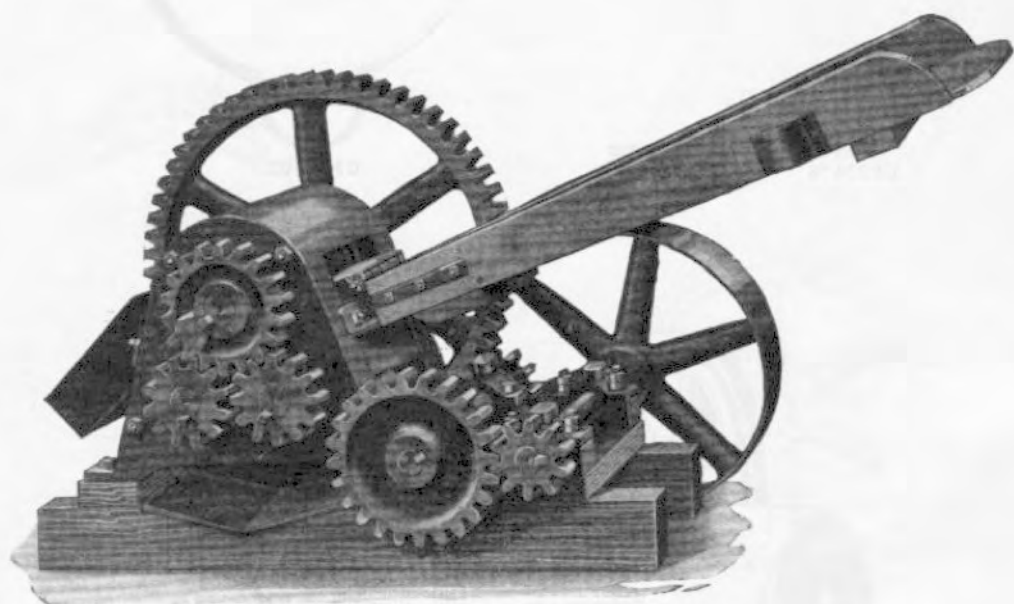
No. 144A Belt-Power Cane Mill (Gear covers are left off on this cut to better illustrate the gears)
