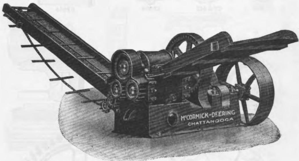
No. 92 Belt-Power Cane Mill.
